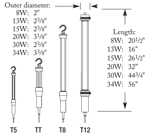
Fluorescent work light with pre-wired K&H Light-Duty Cord Reel
